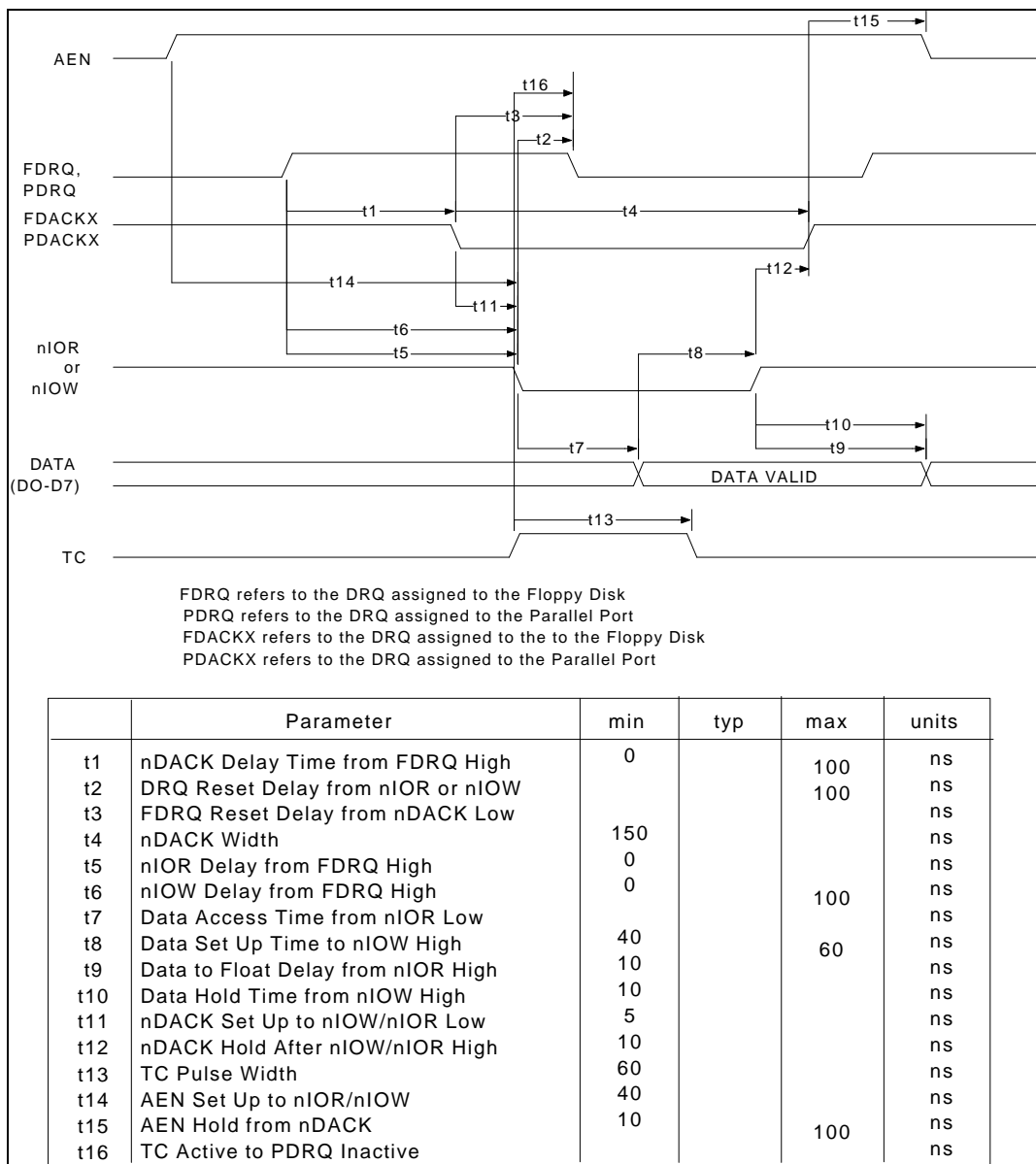
FIGURE 6 - DMA TIMING
